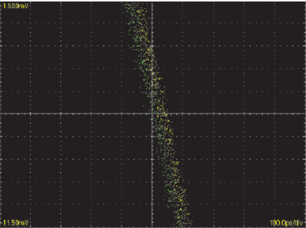
Figure 2. Using the SMC T-Clock synchronization, two or more NI 5412 generators can achieve less than 20 ps channel-to-channel skew.
