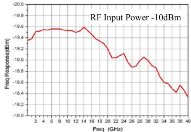
Frequency Response (dBm) VS. Frequency (GHz)
