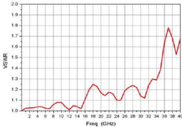
VSWR VS. Frequency (GHz)
