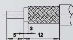
Cable stripping dimensions
