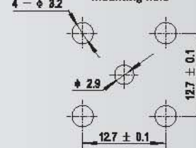
Mounting hole
