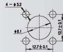
Mounting hole
