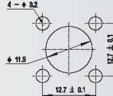
Mounting hole
