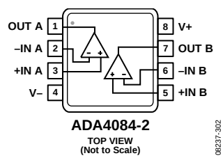
图6. ADA4084-2, 8引脚 MSOP (RM)
