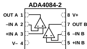
图1. ADA4084-2, 8引脚LFCSP (CP)
