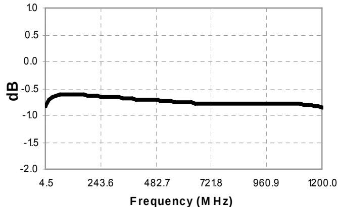
Insertion Loss 2: (Pin 6 to Pin 3)
