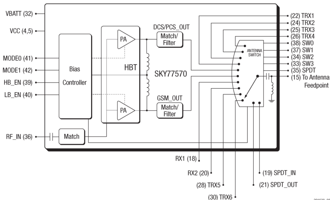
Figure 1. SKY77570 Functional Block Diagram
