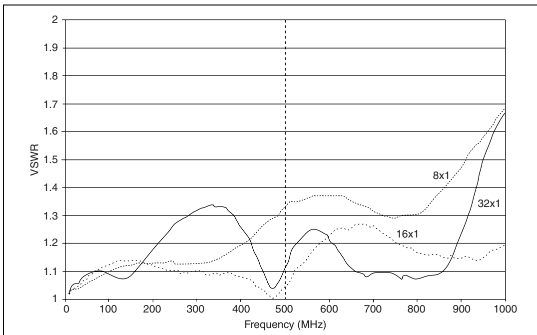
Figure 2. Typical VSWR
