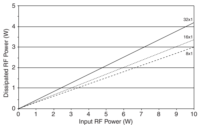
Figure 5. Maximum RF Power Dissipation per Channel
