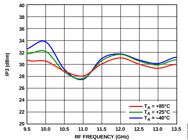
Figure 72. Output IP3 vs. RF Frequency at Various Temperatures, LO = 2 dBm, V_{DLOX} = 2.4 V
