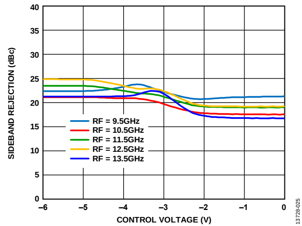
Figure 25. Sideband Rejection vs. Control Voltage at Various RF Frequencies, LO = 2 dBm, V_{DLOx} = 2.4 V
