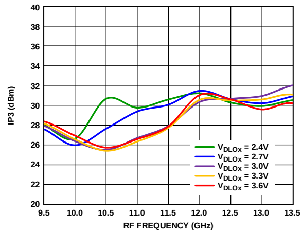
Figure 54. Output IP3 vs. RF Frequency at Various V_{DLOx} , LO = 2 dBm
