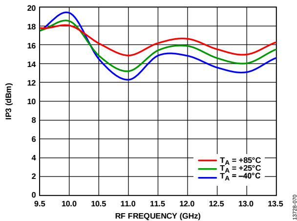
Figure 69. Input IP3 vs. RF Frequency at Various Temperatures, LO = 2 dBm, V_{DLOX} = 2.4 V
