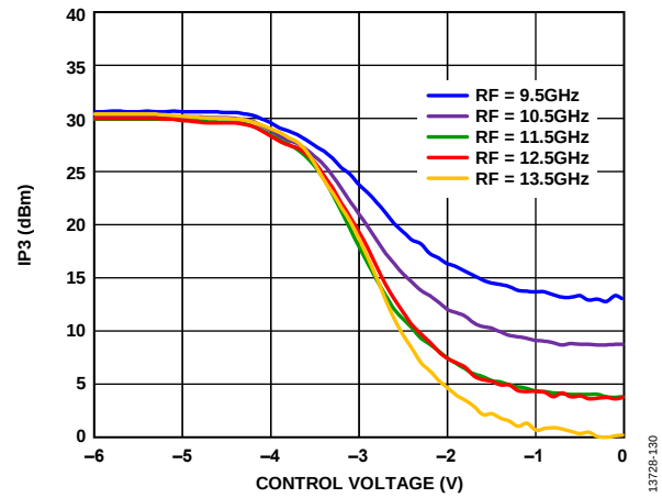
Figure 128. Output IP3 vs. Control Voltage at Various RF Frequencies, LO = 2 dBm, V_{DLOx} = 2.7 V
