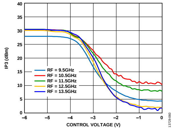
Figure 59. Output IP3 vs. Control Voltage at Various RF Frequencies, LO = 2 dBm, V_{DLOX} = 2.4 V
