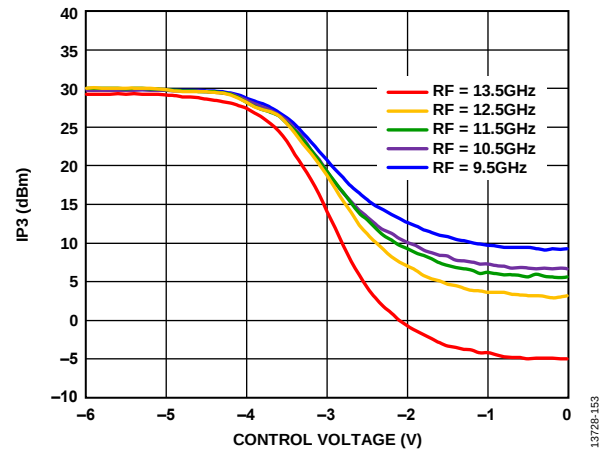
Figure 151. Output IP3 vs. Control Voltage at Various RF Frequencies, LO = 2 dBm, V_{DLOx} = 2.7 V
