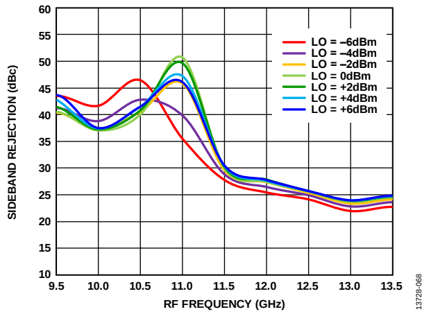
Figure 67. Sideband Rejection vs. RF Frequency at Various LO Powers, V_{DLOX} = 2.4 V
