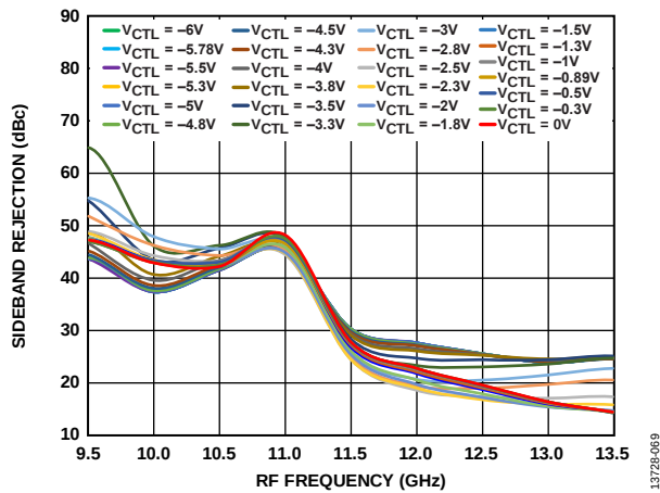
Figure 68. Sideband Rejection vs. RF Frequency at Various Control Voltages ( V_{CTL} ), LO = 2 dBm, V_{DLOX} = 2.4 V
