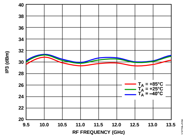
Figure 26. Output IP3 vs. RF Frequency at Various Temperatures, LO = 2 dBm, V_{DLOx} = 2.4 V
