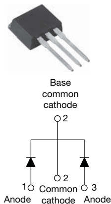
TO-262
