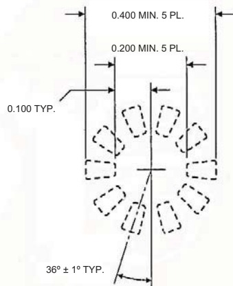
RECOMMENDED PAD LAYOUT See Notes 5 and 6
