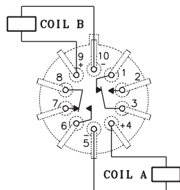
SCHEMATIC-TERMINAL VIEW PIN NUMBERS ARE FOR REFERENCE ONLY (NOT MARKED ON RELAY) COIL A SHOWN LAST ENERGIZED
