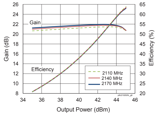
CW Performance V_{DD} = 28 \text{ V} , I_{DQ} = 170 \text{ mA}
