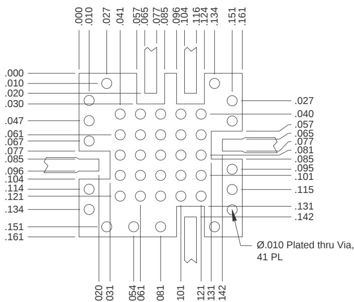
PCB Footprint Drawing
