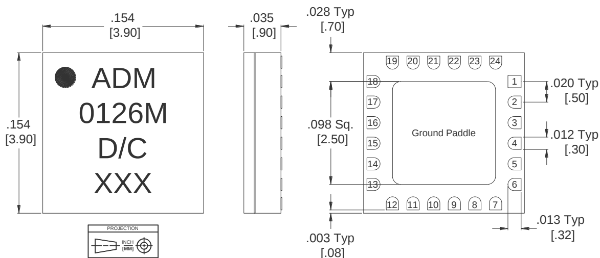
Outline Drawing
