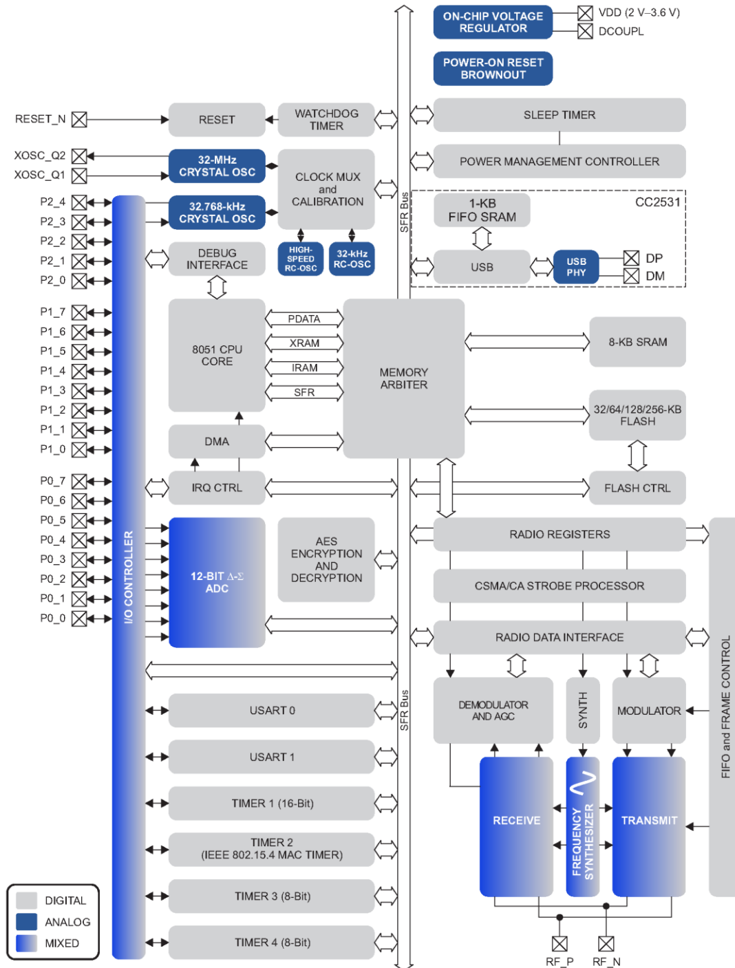
Figure 4 CC2530 SOC Block Diagram
