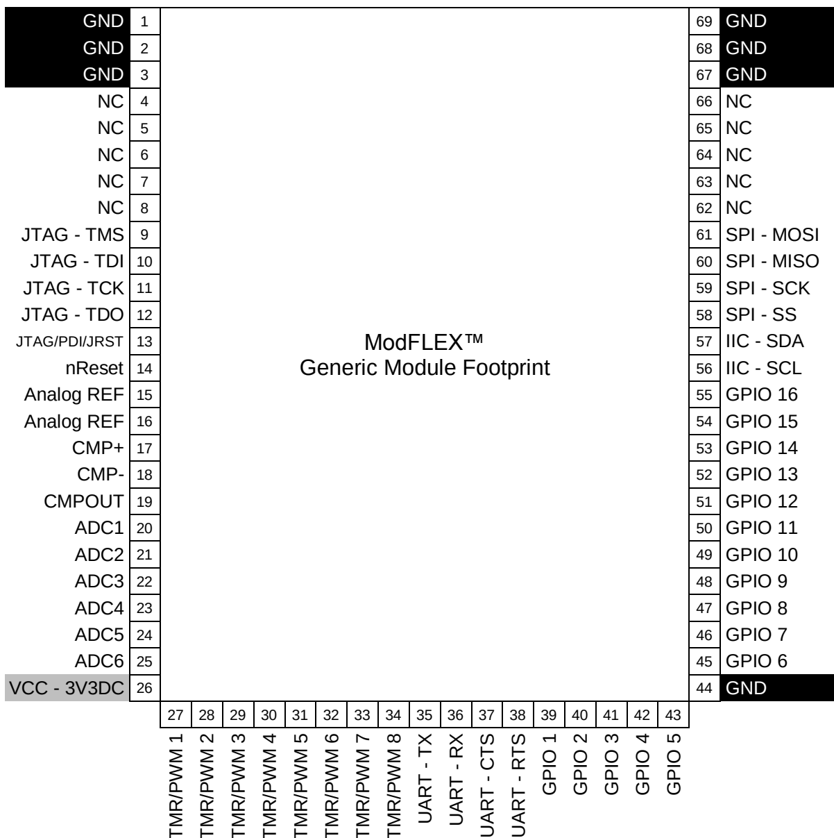
Figure 9 ModFLEX™ Generic Module Footprint
