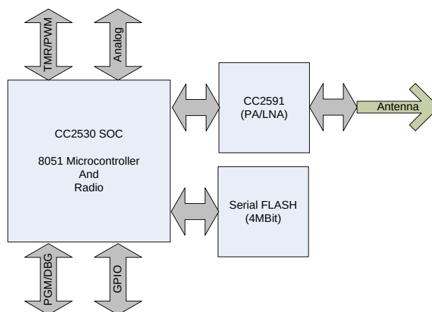
Figure 1 ProFLEX01-SOC Module Block Diagram – High-Level
