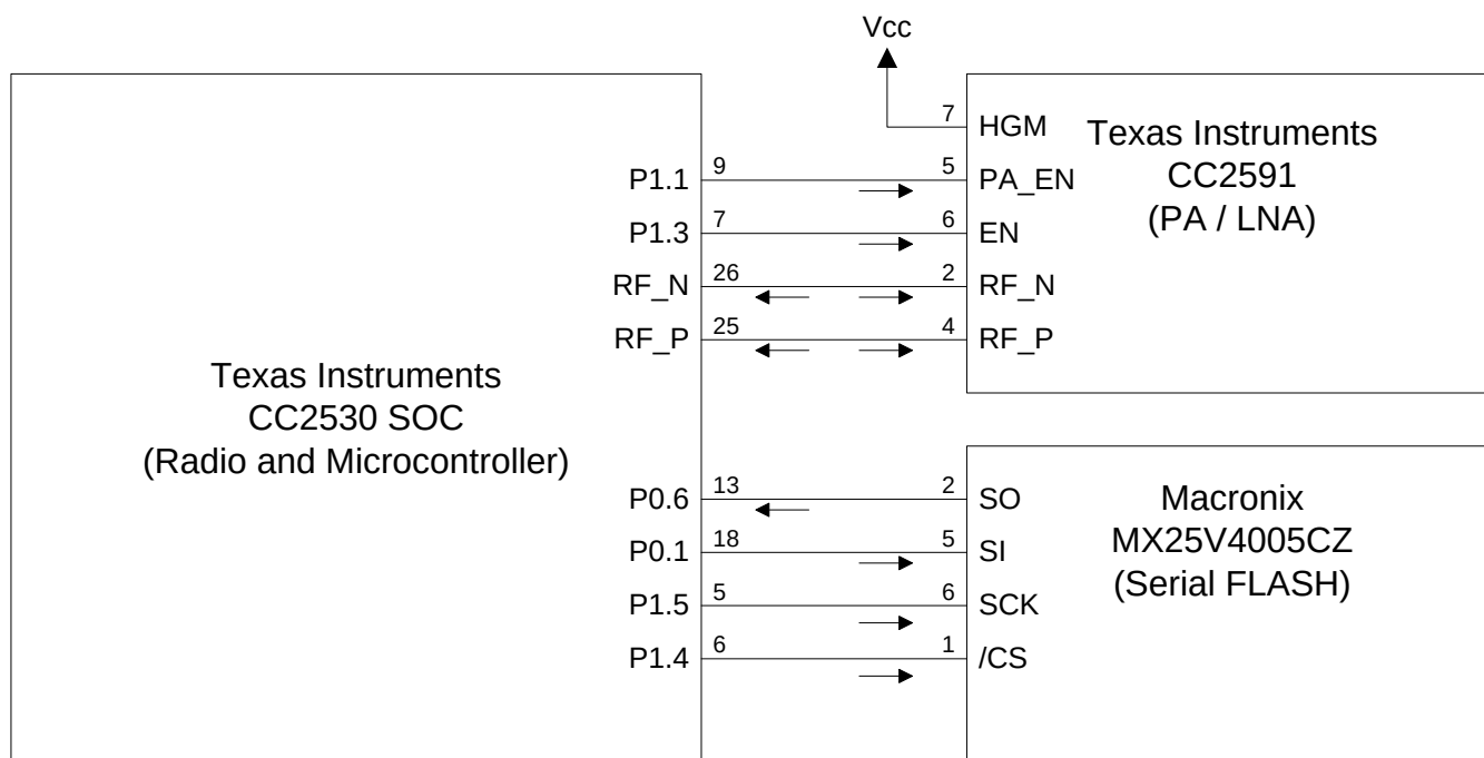
Figure 3 ProFLEX01-SOC Module Block Diagram – Internal Interconnects
