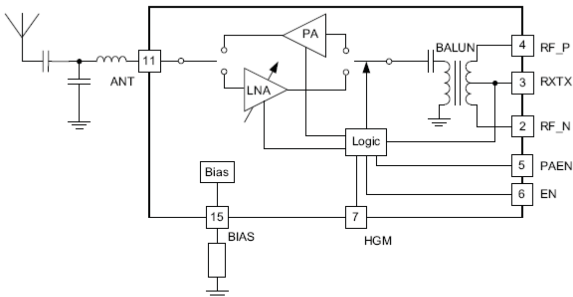
Figure 5 CC2591 Block Diagram
