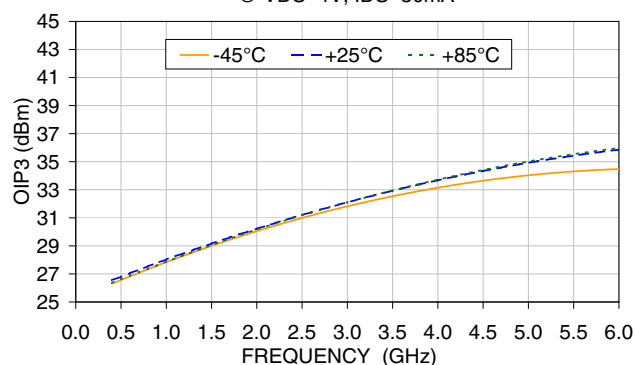
OIP3 vs FREQUENCY & TEMPERATURE (1) @ VDS=4V, IDS=30mA
