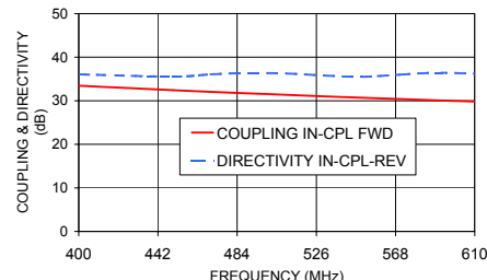
SYBD-30-62HP+ COUPLING & DIRECTIVITY
