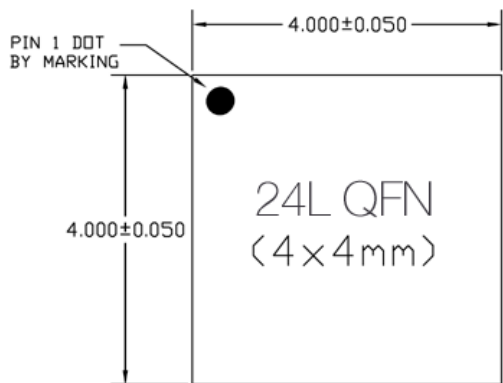
Figure 19. Package Drawing
