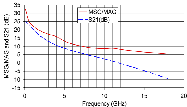
MAXIMUM STABLE GAIN (MSG)/MAXIMUM AVAILABLE GAIN (MAG) vs. FREQUENCY V_{DS}=3V & I_{DS}=15mA
