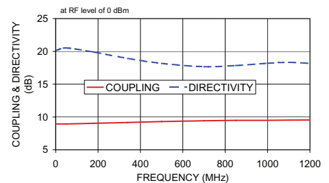
DBTC-9-4-75L+ COUPLING & DIRECTIVITY
