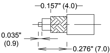
STRIPPING DIMENSIONS
