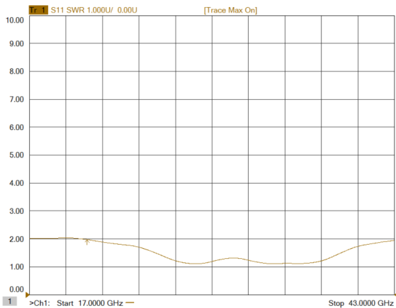
Figure 1-4: ERZ-HPA-1700-4300-22 Input Matching
