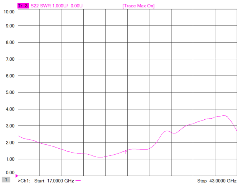
Figure 1-5: ERZ-HPA-1700-4300-22 Output Matching
