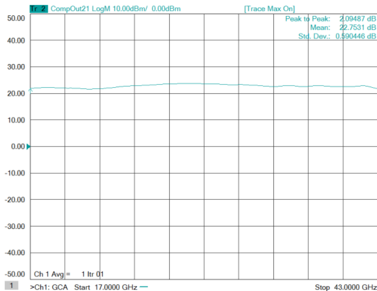
Figure 1-1: ERZ-HPA-1700-4300-22 Psat
