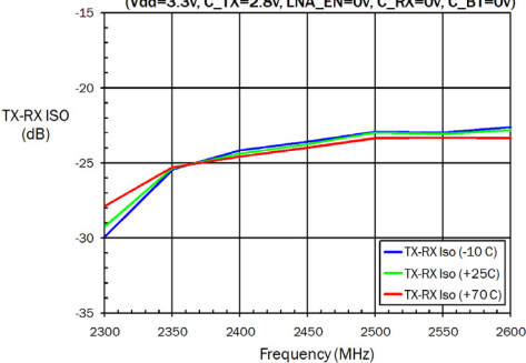
RF5501: TRANSMIT TO RECEIVE ISOLATION versus FREQUENCY and TEMPERATURE (Vdd=3.3v, C_TX=2.8v, LNA_EN=0v, C_RX=0v, C_BT=0v)
