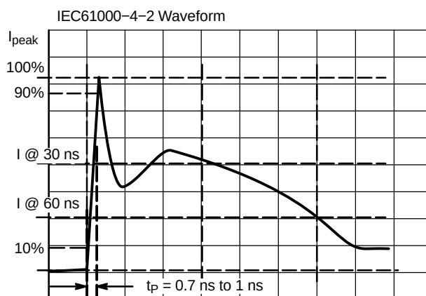
Figure 2. IEC61000-4-2 Spec
