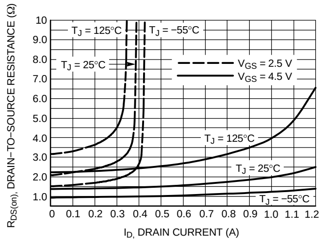
Figure 11. On-Resistance vs. Drain Current and Gate Voltage
