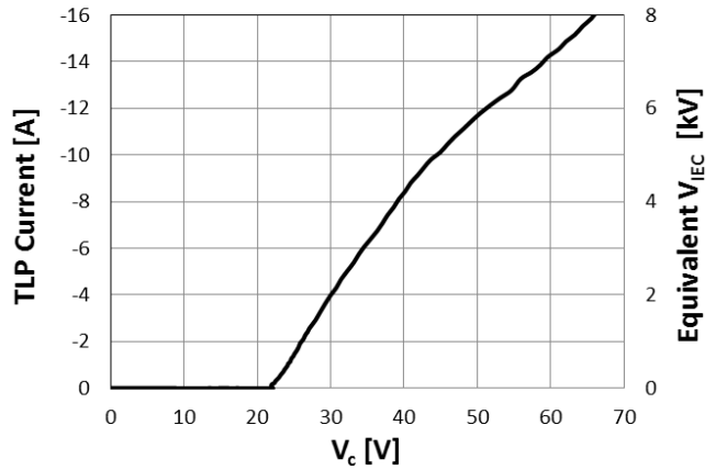
Figure 5. Negative TLP I-V Curve
