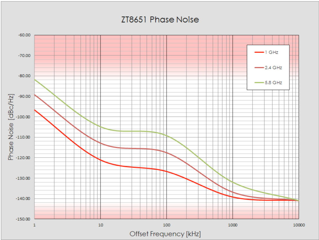
Figure 5: Typical Phase Noise (PXle)
