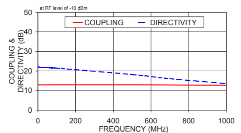
TCD-13-4+ COUPLING & DIRECTIVITY
