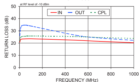
TCD-13-4+ RETURN LOSS
