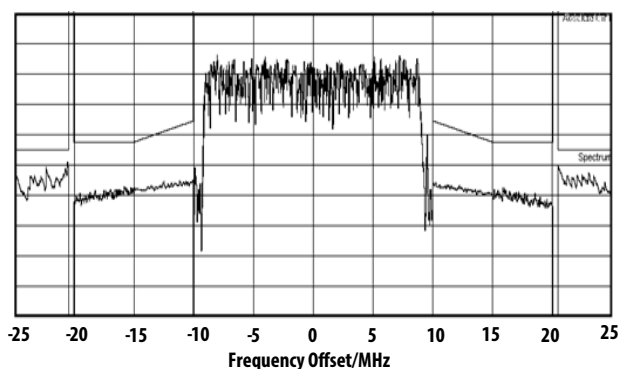
Figure 21. SEM at Pout=29dBm @ 1.842GHz
