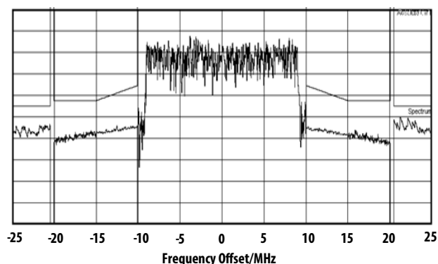
Figure 22. SEM at Pout=29dBm @ 1.87GHz
