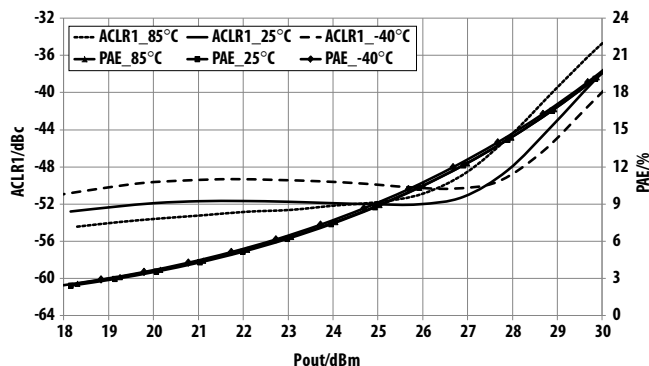
Figure 8. Over-temperature ACLR1, PAE vs Pout @ 1.815GHz V_{dd}=V_{ddBias}=5.5V operating voltage
