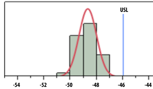
Figure 4. ACLR1 at Pout=27.0dBm, Nominal = -48.7dBc
