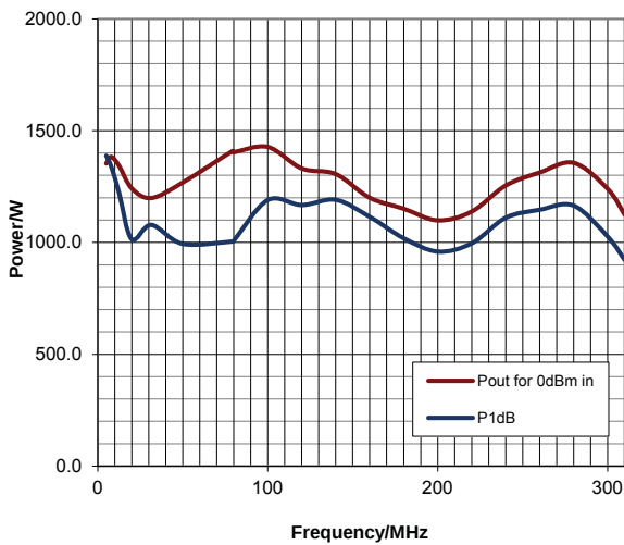
Typical peak envelope power plots
