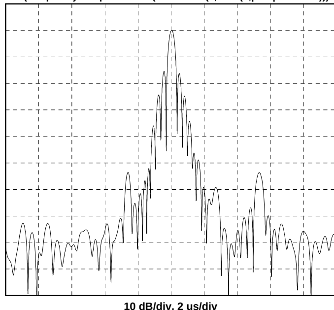
Impulse Response
