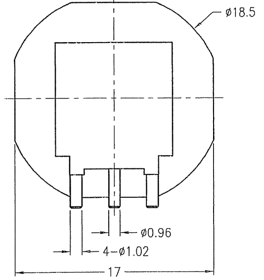
RECOMMENDED MOUNTING HOLE
