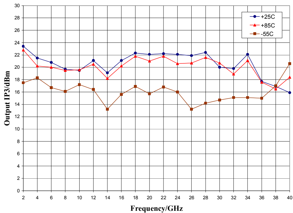
Output IP3 vs. Temperature, V_{dd} = 4\text{ V} , V_{gg} = 3\text{ V}
