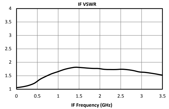
Typical Performance
