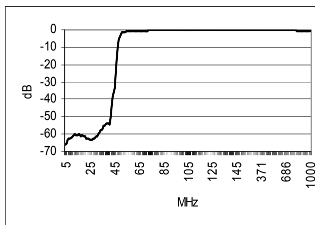
High Pass Filter Insertion Loss
