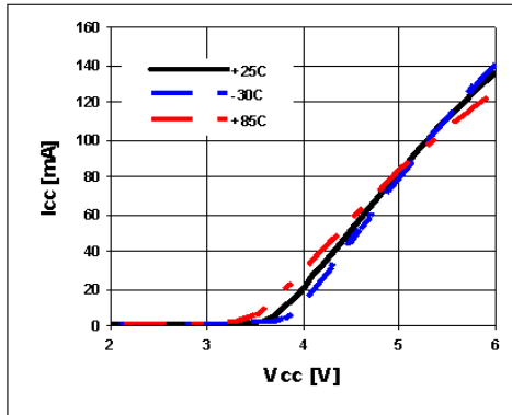
V-I Characteristics
