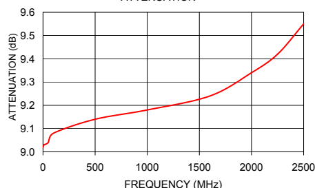
LAT-9+ ATTENUATION
