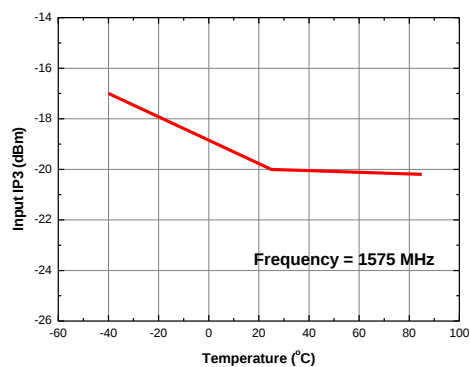
Input IP3 vs. Temperature
