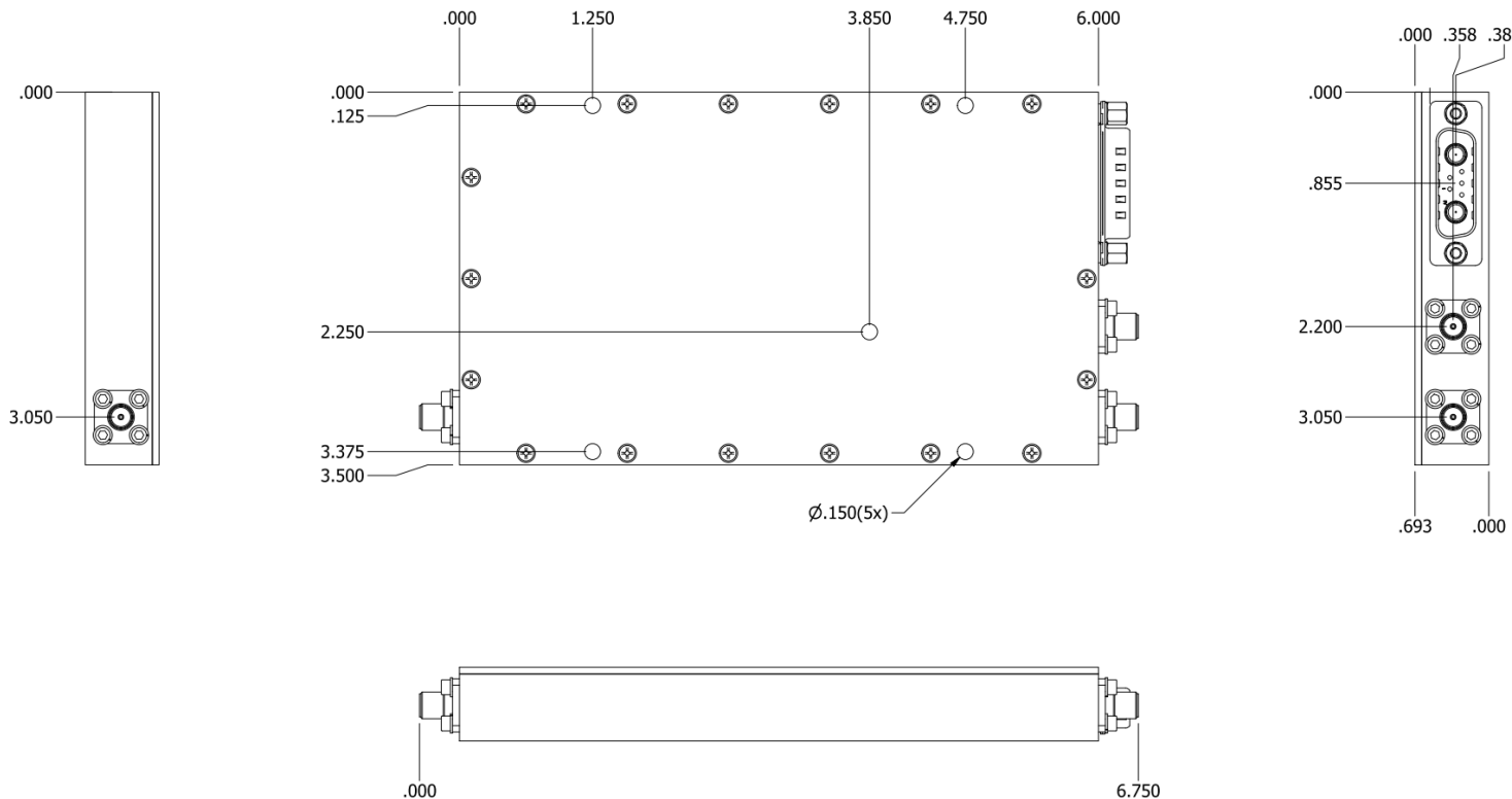
OUTLINE DRAWING
