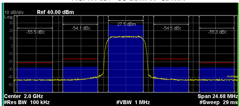
ACPR PLOT - 35 dBm W-CDMA
