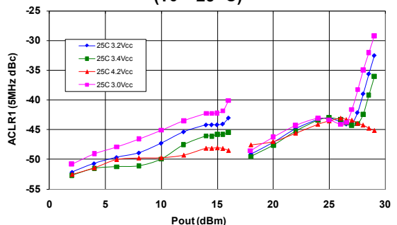
Figure 9: WCDMA ACLR1 (dBc) over Voltage ( T_c = 25\text{ }^{\circ}\text{C} )
