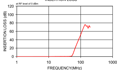
SCLF-45 INSERTION LOSS
