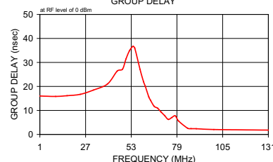
SCLF-45 GROUP DELAY
