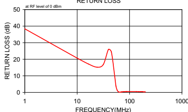
SCLF-45 RETURN LOSS
