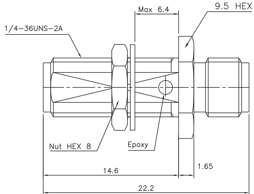
SMA Bulkhead JACK TO JACK -ADAPTOR
