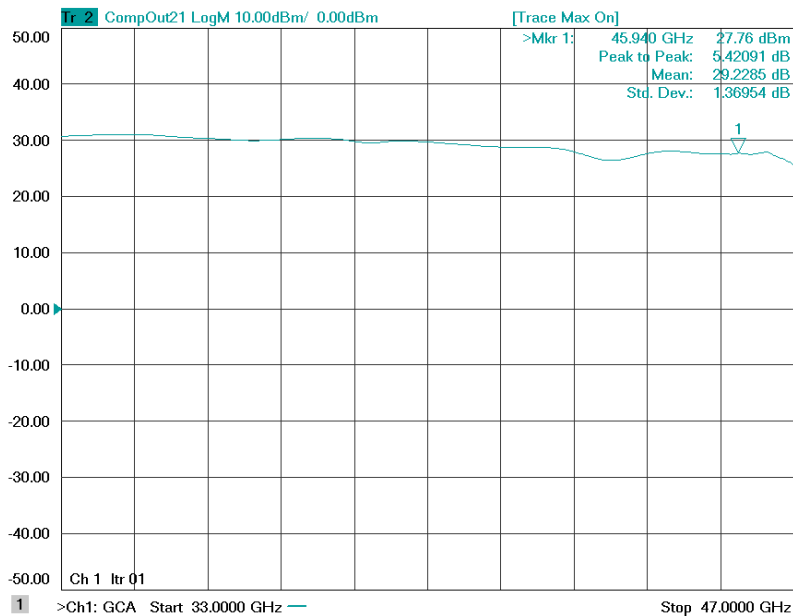
Figure 1-1: ERZ-HPA-3300-4700-29 Psat
