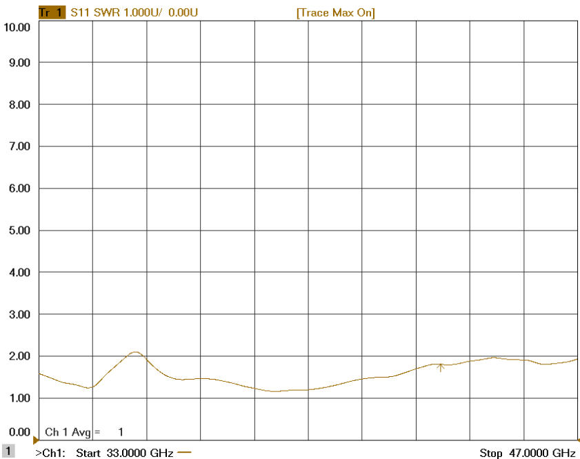
Figure 1-4: ERZ-HPA-3300-4700-29 Input Matching
