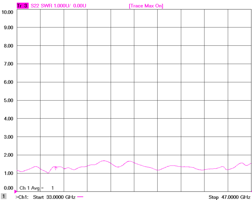
Figure 1-5: ERZ-HPA-3300-4700-29 Output Matching
