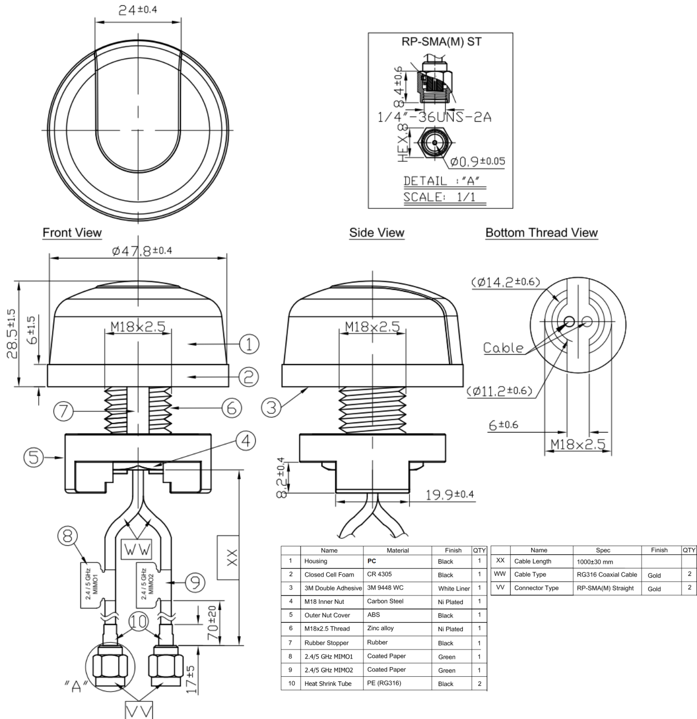
Figure 23. Antenna Drawing
