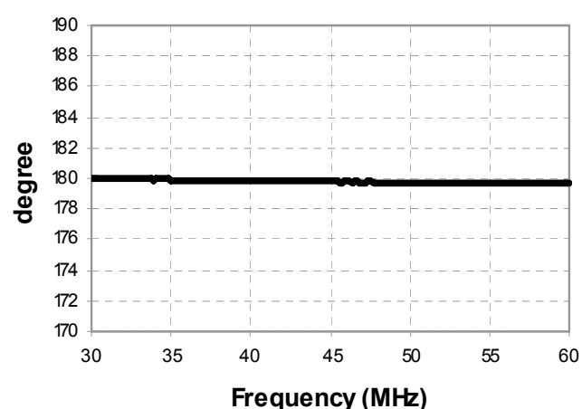
Phase Balance
