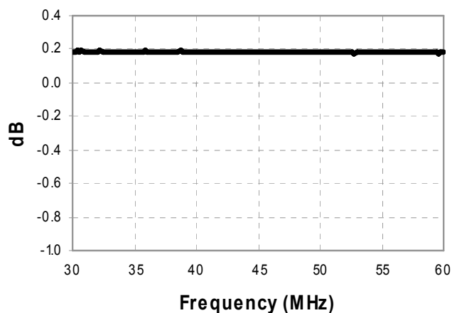
Amplitude Balance
