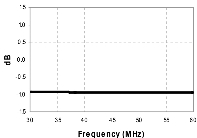
Amplitude Balance
