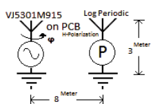
Fig. 3 - VJ5301M915 PCB Mounting and Coordinate Directions
