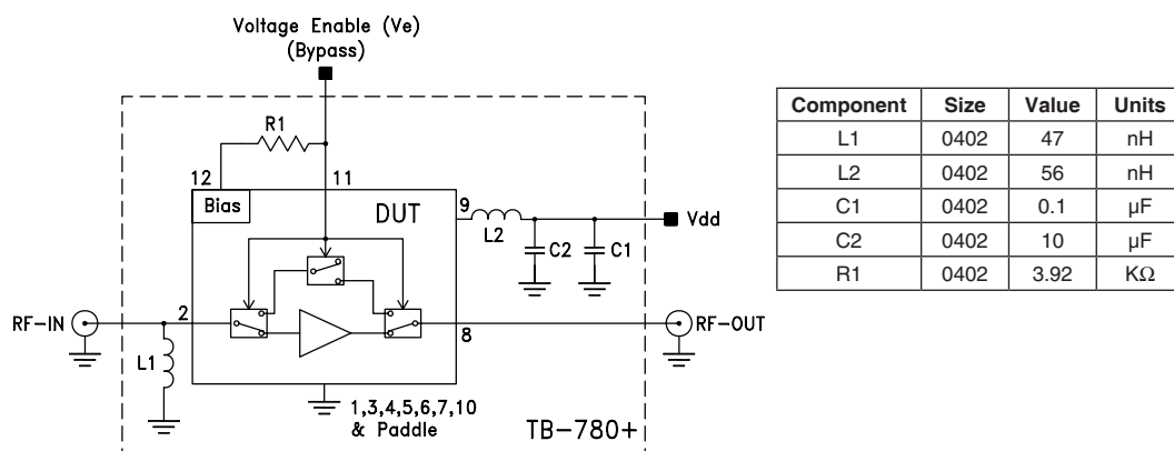
Fig 1. Block diagram of Test Circuit used for characterization. (DUT soldered on Mini-Circuits Characterization test board TB-780+) Gain, Return loss, Output power at 1dB compression (P1 dB), output IP3 (OIP3) and noise figure measured using Agilent's N5242A PNA-X microwave network analyzer.
