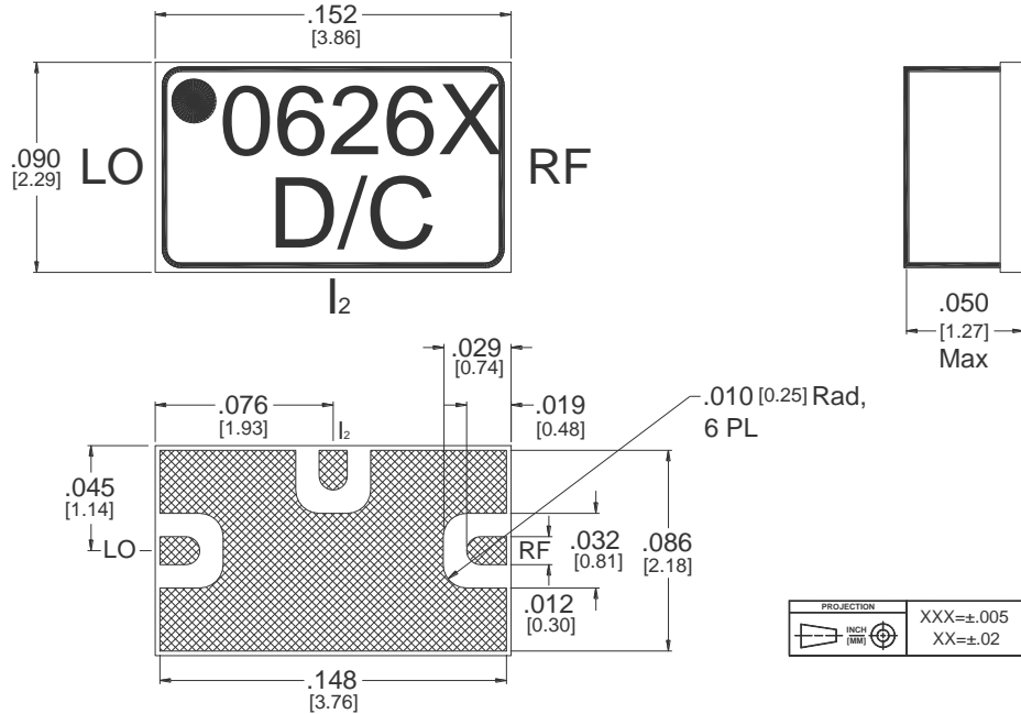
Outline Drawing – SM-2 Package
