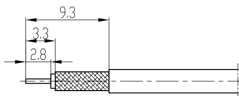
剥线尺寸 stripping dimension
