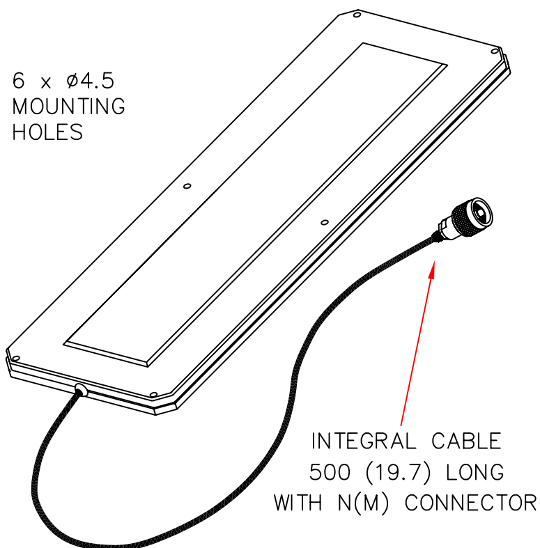
ISOMETRIC VIEW
