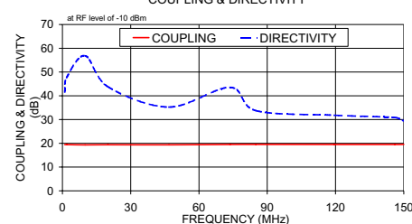
ZDC-20-3-75 COUPLING & DIRECTIVITY
