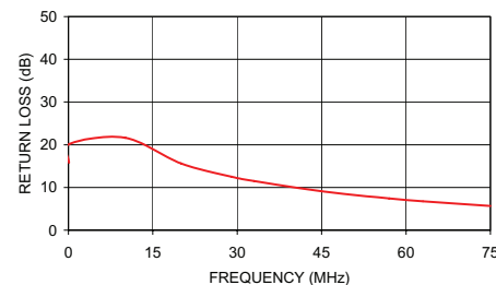
ADT16-6T INPUT RETURN LOSS
