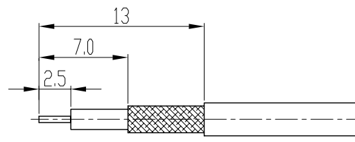
剥线尺寸 stripping dimension
