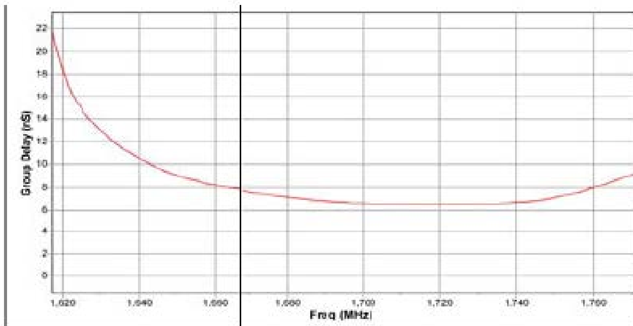
Group Delay
